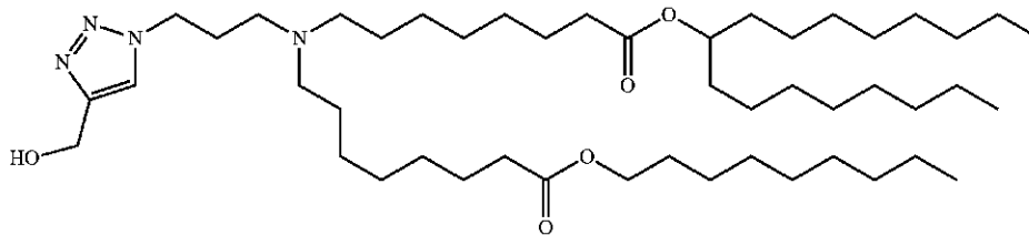
Chemical Formula: \text{C}_{48}\text{H}_{92}\text{N}_4\text{O}_5 Molecular Weight: 805.29
