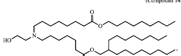
(Compound 143)
