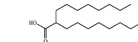
Chemical Formula: C 18 H 36 O 2 Molecular Weight: 284.48
