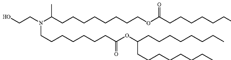
Heptadecan-9-yl 8-((2-hydroxyethyl)(10-(octanoyloxy)decan-2-yl)amino)octanoate
