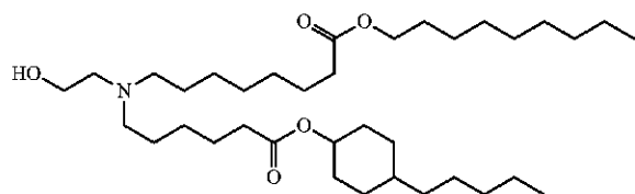
Chemical Formula: \text{C}_{36}\text{H}_{69}\text{NO}_5 Molecular Weight: 595.950
