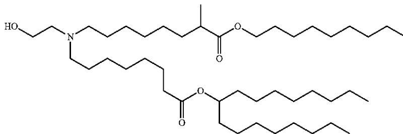
Chemical Formula: C_{45}H_{89}NO_5 Molecular Weight: 724.209
