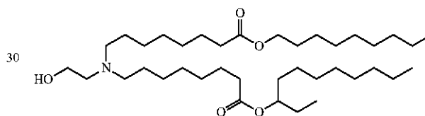
Chemical Formula: C_{38}H_{75}NO_5 Molecular Weight: 626.02
