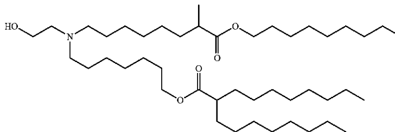
7-((2-Hydroxyethyl)(7-methyl-8-(nonyloxy)-8-oxooctyl)amino)heptyl 2-octyldecanoate
