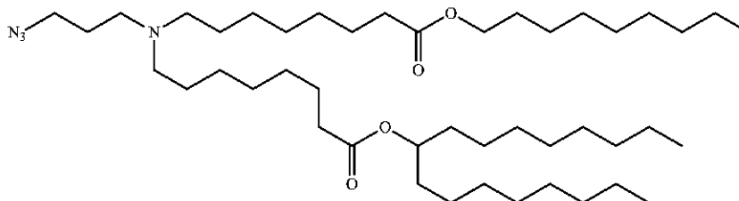
Heptadecan-9-yl 8-((3-azidopropyl)(8-nonyloxy)-8-oxooctyl)amino)octanoate
