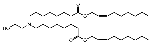
Chemical Formula: C 36 H 67 NO 5 Molecular Weight: 593.93
