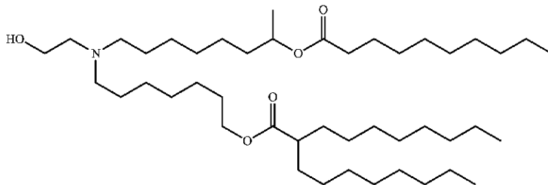
Chemical Formula: C_{45}H_{89}NO_5 Molecular Weight: 724.209
