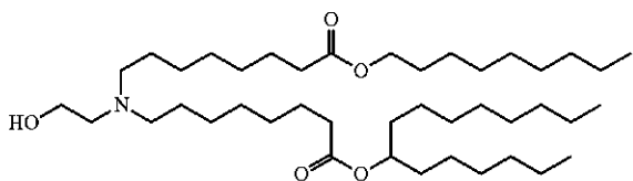
Chemical Formula: C_{42}H_{83}NO_5 Molecular Weight: 682.13
