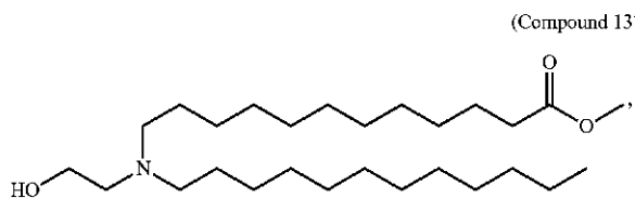
(Compound 139)
