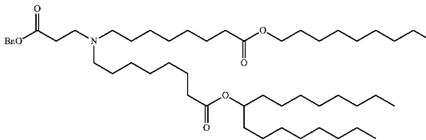
Heptadecan-9-yl 8-((3-(benzyloxy)-3-oxopropyl)(8-(nonyloxy)-8-oxooctyl)amino)octanoate
