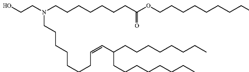
Nonyl (Z)-8-((2-hydroxyethyl)(10-octyl)amino)octanoate
