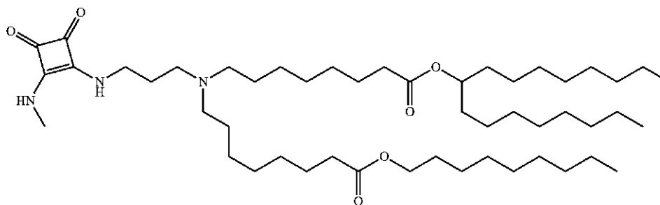
Chemical Formula: C_{50}H_{93}N_3O_6 Molecular Weight: 832.31
