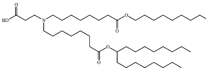
3-((8-(Heptadecan-9-yloxy)-8-oxooctyl)(8-(nonyloxy)-8-oxooctyl)amino)propanoic acid
