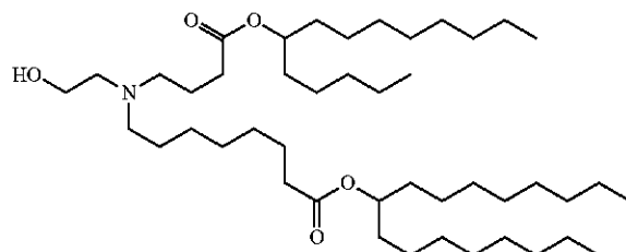
Chemical Formula: C 45 H 89 NO 5 Molecular Weight: 724.209
