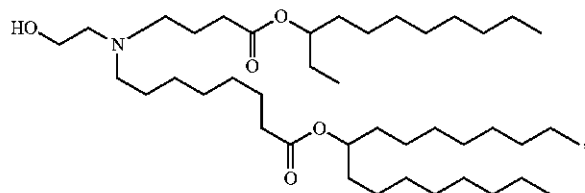
(Compound 72)
