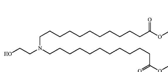
Chemical Formula: C 28 H 55 NO 5 Molecular Weight: 485.75
