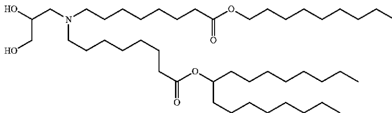
Chemical Formula: C 45 H 89 NO 6 Molecular Weight: 740.21
