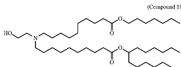
(Compound 185)
