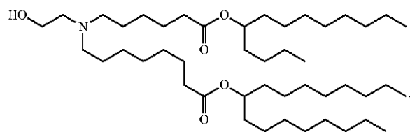
(Compound 77)
