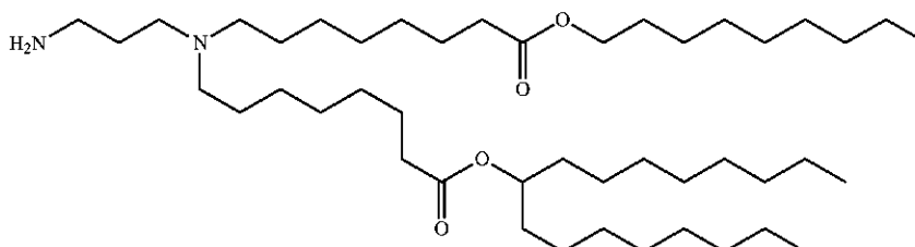
Heptadecan-9-yl 8-((3-aminopropyl)(8-nonyloxy)-8-oxooctyl)amino)octanoate
