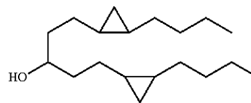
Chemical Formula: C 19 H 36 O Molecular Weight: 280.496
