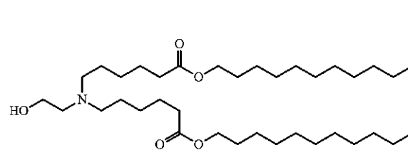
Chemical Formula: C 36 H 71 NO 5 Molecular Weight: 597.97
