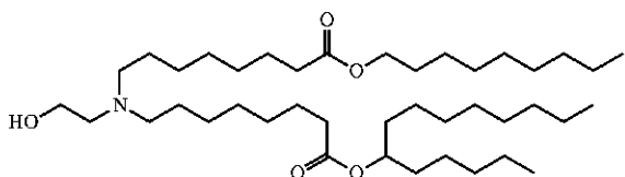
Chemical Formula: C_{41}H_{81}NO_5 Molecular Weight: 668.10
