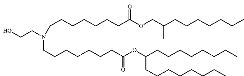
(Compound 185)
