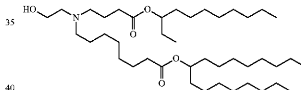
Chemical Formula: C 42 H 83 NO 5 Molecular Weight: 682.13
