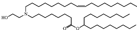
Chemical Formula: C_{45}H_{89}NO_5 Molecular Weight: 692.21
