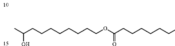
9-Hydroxydeacyl octanoate
