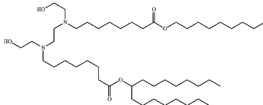
Chemical Formula: C 48 H 96 N 2 O 6 Molecular Weight: 797.304
