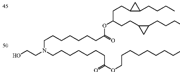
Chemical Formula: C 46 H 87 NO 5 Molecular Weight: 734.204
