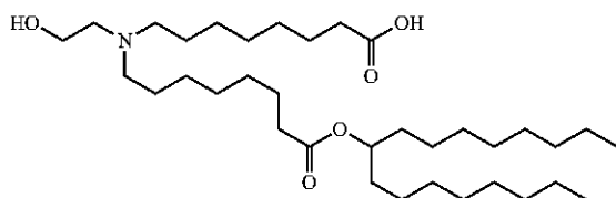
Chemical Formula: C_{35}H_{69}NO_5 Molecular Weight: 583.939
