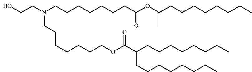
(Compound 136)
