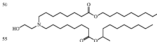
Chemical Formula: C_{37}H_{73}NO_5 Molecular Weight: 611.99
