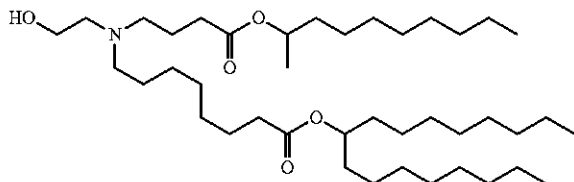
Chemical Formula: C 41 H 81 NO 5 Molecular Weight: 667.61
