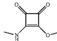
Chemical Formula: C_6H_7NO_3 Molecular Weight: 141.13
