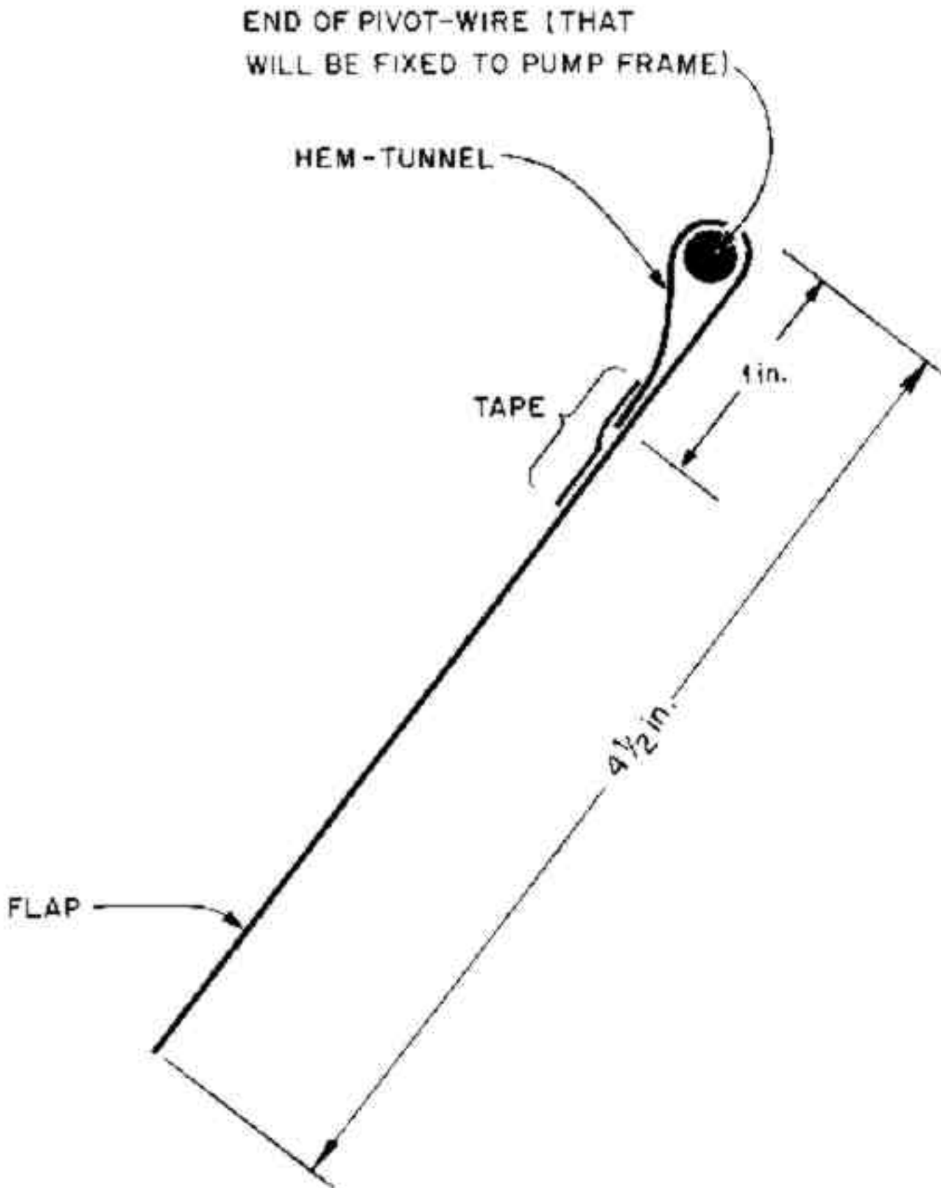
Fig. 7. End view.
